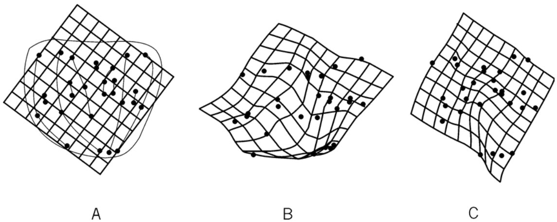
Fig. 4. The transformation grid showing change of dental crown pattern in consensus configuration (A) as it is transformed into Muscardinus (B) and Myomimus (C) patterns
